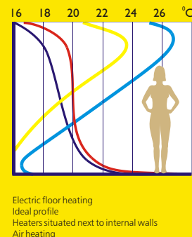
VERTICAL DISTRIBUTION OF TEMPERATURE IN A ROOM FOR THE VARIOUS TYPES OF HEATING
